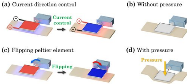
Figure 6: Operation overview of the two variables used in the user study: (a, c) Thermal stimulation methods, (b, d) Presence of pressure feedback.
