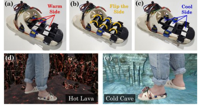
Figure 13: Flip-Pelt system applied in VR shoes: (a) Contact with a warm surface, (b) Peltier element rotating within the sole space, (c) Contact with a cool surface, (d, e) Example scenarios in VR contents.
