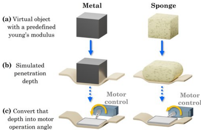
Figure 5: Virtual pressure simulation overview: (a) Virtual objects with predefined Young’s modulus (e.g., Metal, Sponge), (b) Skin penetration depth calculation, (c) Servo motor angle adjustment based on calculated penetration depth.
