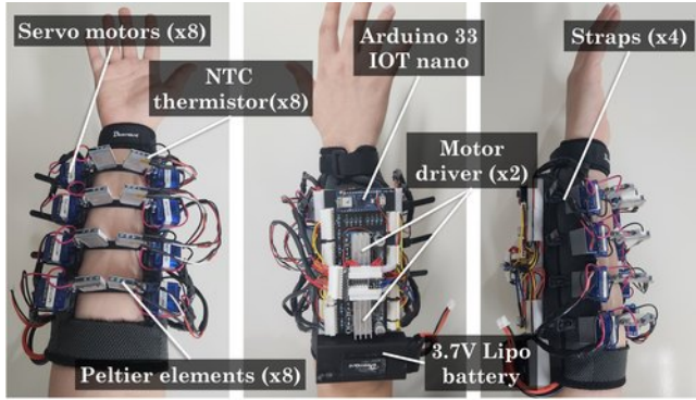
Figure 2: Hardware configuration of the Flip-Pelt device. (Left) Front view showing servo motors, temperature sensors, and peltier elements. (Center) Back view showing the battery, motor driver, and microcontroller.
