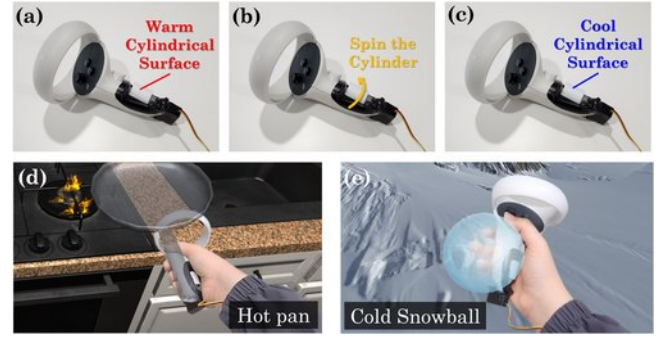
Figure 14: Flip-Pelt system applied in VR controller: (a) Contact with a warm cylindrical surface, (b) Peltier element spinning within the controller, (c) Contact with a cool cylindrical surface, (d, e) Example scenarios in VR contents.
