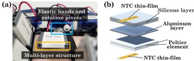
Figure 3: Detailed design of the dual-sided peltier element: (a) Utilizing elastic bands and rotation pivots, (b) Multi-layer composition.
