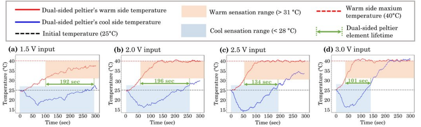
Figure 4: Measurement of time-dependent temperature and lifetime of the dual-sided peltier element (input range 1.5–3.0V)
